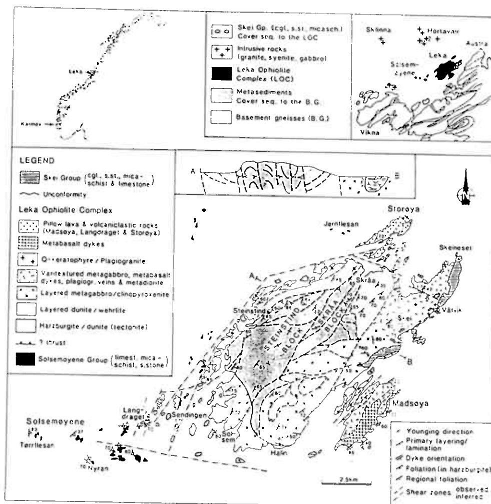
FIG. 1. Simplified geological map of the Leka Ophiolite Complex (From Furnes et al. 1988)
