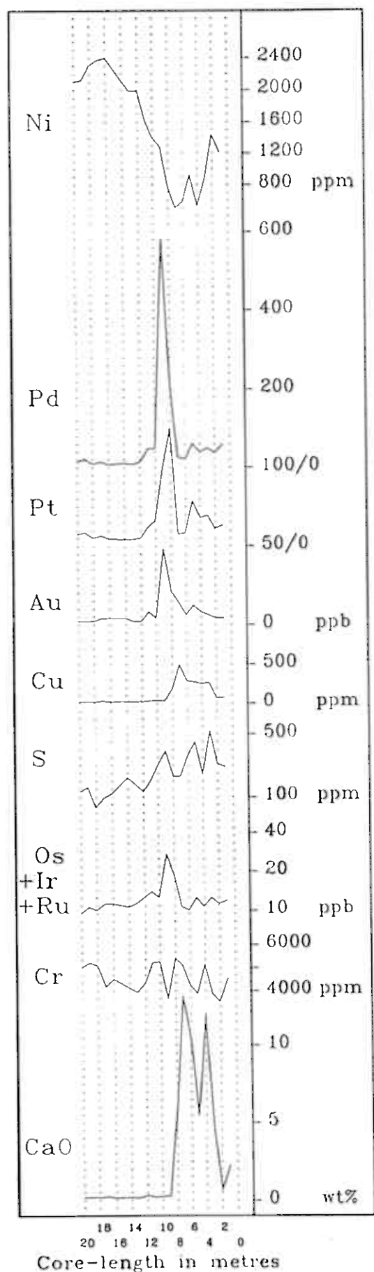
FIG. 11. Compositional variations with height across the base of R2 along profile C (core 88B6).
