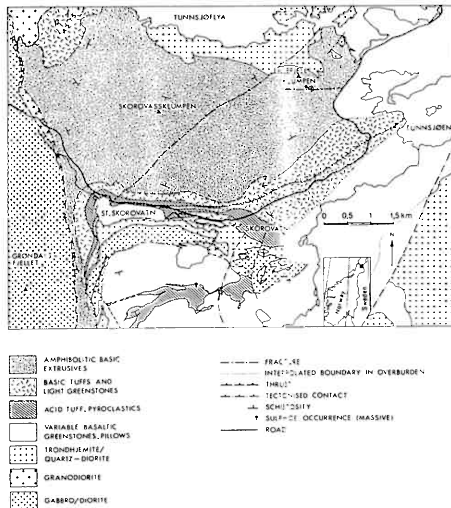
Fig. 1. Simplified geological map of the Lillefjellklumpen-Skorovåren area, based on Hallis et al. (1977), Kollung (1979) and A. Reinsbakken (pers. comm. 1984).
