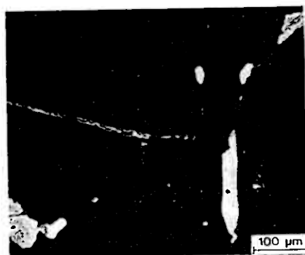
Fig. 3. Three merenskyite grains (white) occurring as: (1) inclusion in pyrrhotite (dark grey); (2) on grain boundary pyrrhotite/pyrrhotite; and (3) exsolved from chalcopyrite (grey). Backscatter electron image.
