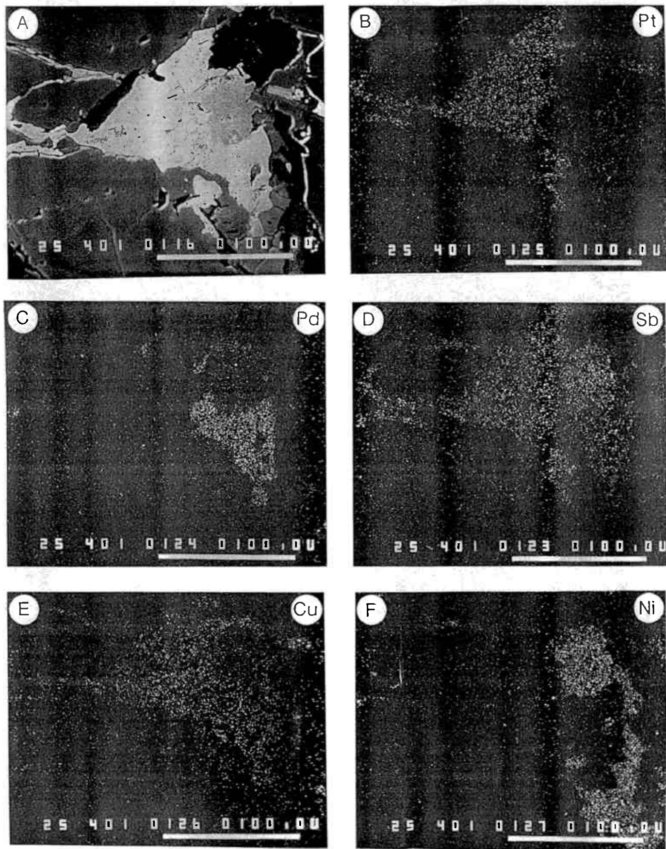
FIG.28. SEM back-scatter picture of composite PGM. B-F show single element scans for Pt, Pd, Sb, Cu, and Ni respectively. The composite grain is composed of domains of Pt-Cu, Pt-Sb, Pd, Sb, Ni-Sb and Ni-As.
