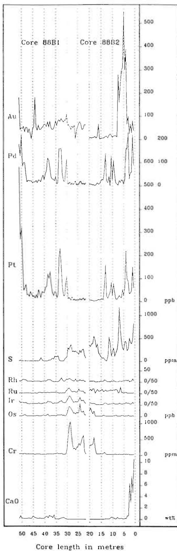
FIG. 12. Geochemical variations with height across and above the main chromitite horizon along profile A (core 88B1 and 88B2).
