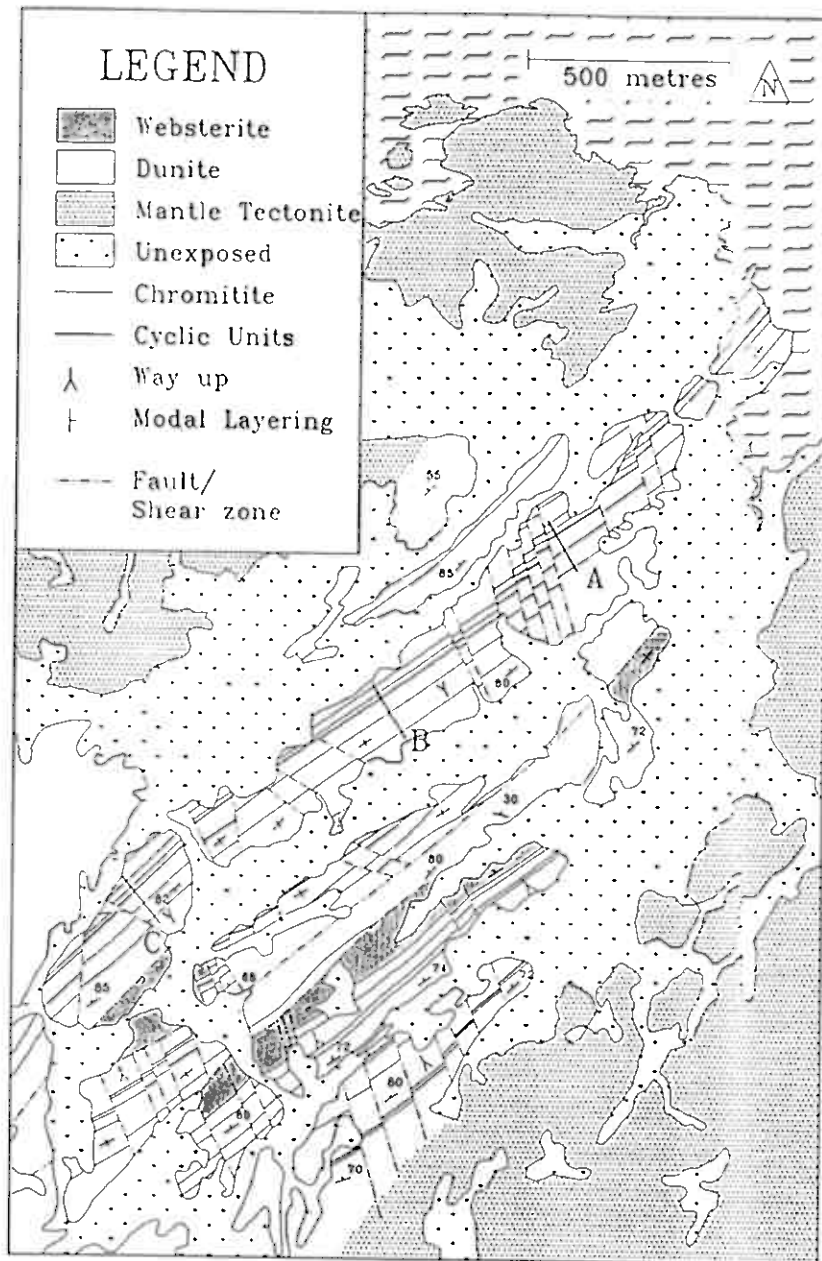
FIG. 3. Detailed map of parts of the ultramafic zone of the layered series which show sub-zones of ol- and ol-pyroxene cumulates. Cyclic units are shown within the ol-cumulate sub-zones where they can be defined in the field. The locations of the main geochemical profiles referred to later in the text are marked by A, B, and C.
