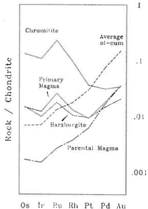
FIG. 34. Chondrite-normalized PGE patterns of the average cyclic units, and estimated parental and primary magma. For further discussion see text.
