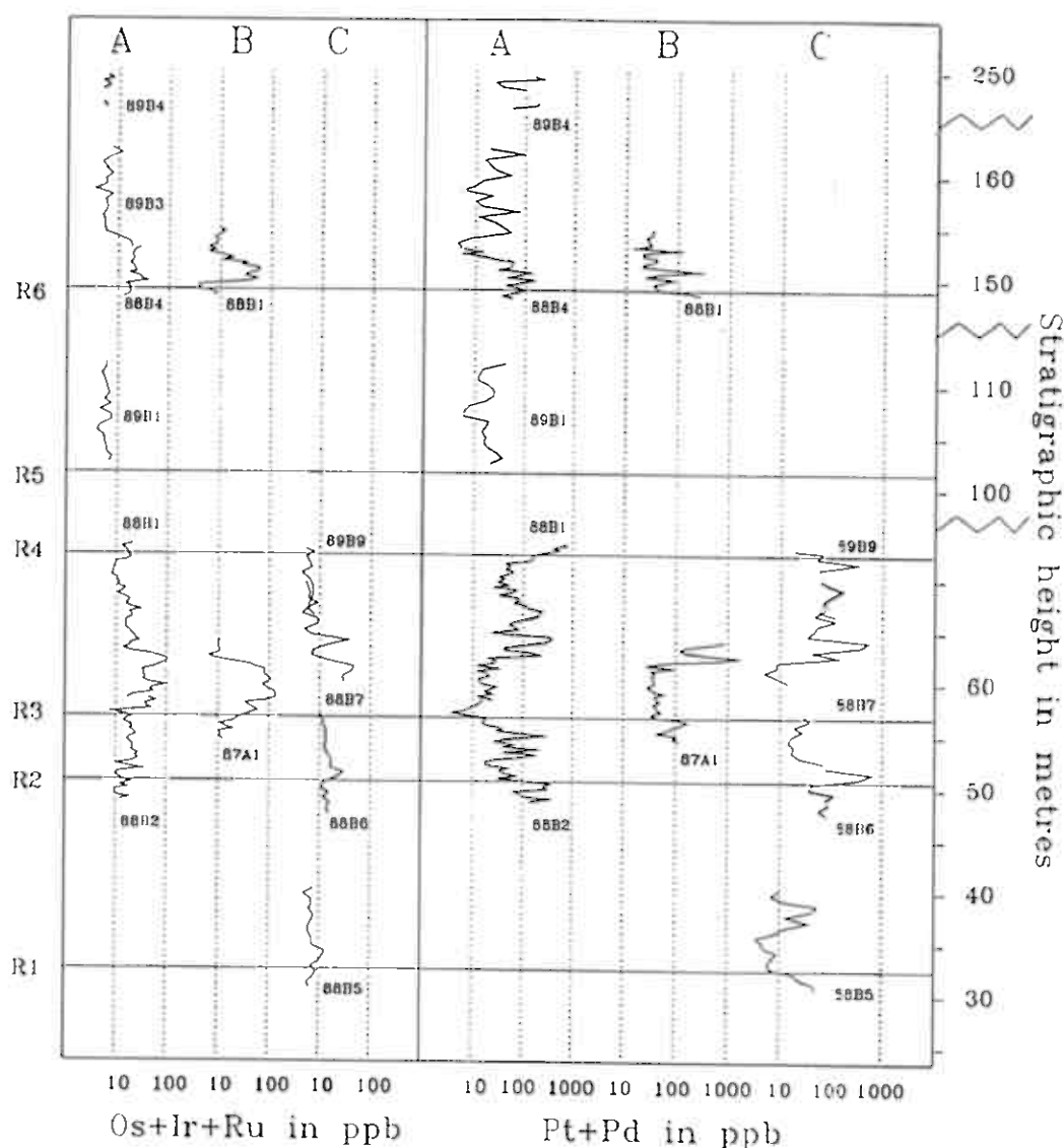
FIG 10.. Compilation of PGE-data from drill-cores taken across the bases of cyclic units along the three major profiles of Fig. 3.
