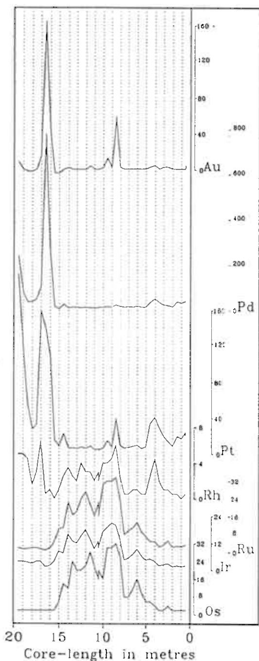
FIG. 14. Variation in PGE contents across the main chromitite horizon in profile B (core 87A1).
