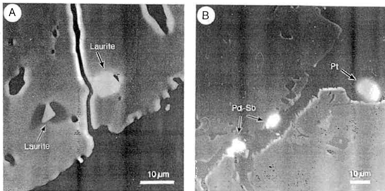
FIG. 26. SEM back-scatter picture of : a) Euhedral laurite (white) in chromite. b) Pd-Sb and native Pt (white) which are positioned interstitially to the chromite grains.
