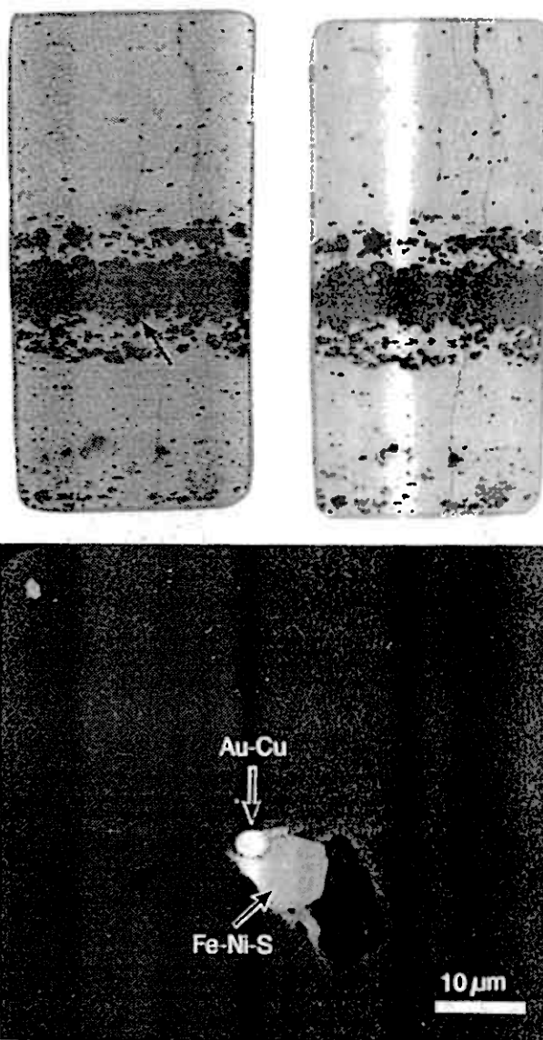
FIG. 21. B-autoradiograph of a stratabound chromitite which show the presence of a B-emitter (see arrow on A) that disappears after 30 days of cooling (B). SEM investigation of the chromite grain demonstrated that the B-emitter probably was a small Au-Cu alloy (C).
