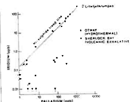
Fig. 6. Pd and Ir contents of major Ni-sulphide deposits of western Australia (Keays et al. 1982) define a Ni-sulphide trend line, close to which analyses from the Lillefjellklumpen deposit plot.
