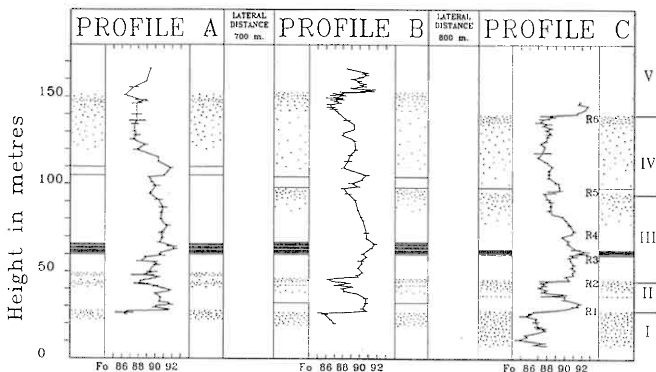
FIG. 4. Cryptic variations across parts of a sub-zone of ol-cumulates. The three profiles are taken across the same cyclic units and are separated laterally by 700 and 800 metres (for the exact location of the profiles see Fig. 3). Cyclic units that can be defined in the field along profile C are marked with I, II, III, IV and V (some of them are less pronounced along profile A). Cryptic reversals in ol-compositions that can be defined in all three profiles are marked by R1, R2, ... (after Pedersen, 1990)
