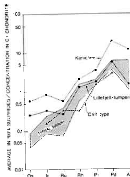
Fig. 5. Chondrite-normalized PGE and Au concentrations for Lillefjellklumpen compared with other gabbro-related deposits (Naldrett 1982) and the Cliff deposit (Gunn et al. 1985).
