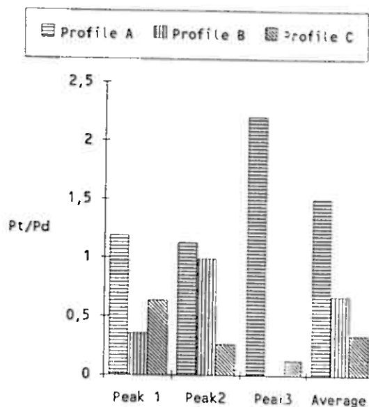
FIG. 15. Histogram that show how the Pt/Pd ratio of the three major PGE-peaks above the main chromitite horizon change laterally. For further discussion see text.
