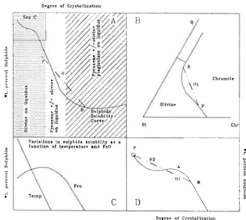
FIG. 31. A) Schematic diagram illustrating assumed evolution in the solubility of iron sulphide with progressive differentiation of basaltic magma (after Naldrett and von Gruenewaldt 1989). B) Phase relations in the system Chromite-olivine-quartz (after Irvine, 1978). C) Schematic diagram illustrating assumed changes in the solubility of sulphide in the magma as a function of variations in the magma-temperature and the FeO content of the magma with progressive differentiation. D) Suggested modifications to the sulphide solubility curve suggested by Naldrett and von Gruenewaldt (1989) (A) which take into account the initial increase in the FeO content of the magma when very magnesian olivines are fractionated
