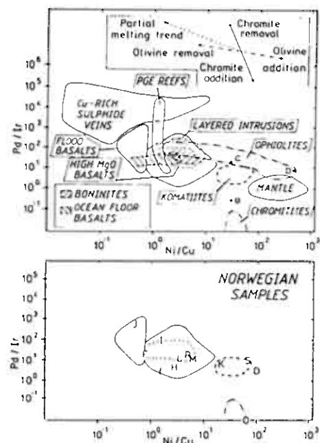
FIG. 3. (a) Metal ratio diagram of Pd/Ir versus Ni/Cu based on literature data for discriminating between the compositional fields of: mantle, komatiites and sulphides associated with them, high MgO-basalts and associated sulphides, ocean-floor basalts, boninites and low-TiO 2 basalts, flood basalts and sulphides associated with them, ophiolites, podiform chromitites from ophiolites, Pt-reefs, layered intrusions of unknown affinity, and Cu-rich sulphides. D = dunites from Thetford ophiolite, B = B-zones of komatiites and C = Cliff locality from Unst. The inset shows the displacement vectors on the diagram for the effects of partial melting of the mantle (dotted), olivine removal or addition (dashed) and chromite removal or addition (solid). (b) Diagram of the Pd/Ir and Ni/Cu ratios of Norwegian mafic and ultramafic rocks compared with selected compositional fields (others left out for the sake of clarity) from Fig. 3(a). Symbols: D = dunites from Leka; K = Karasjok komatiites; S = Rombak komatiites; O = Leka ophiolite chromitite; F = Fiedy ophiolite sulphides; R = Reinford Tholeiitic Intrusion; M = Melkvaun Alkaline Intrusion; L = Lille Kuljord Tholeiitic Intrusion; J = Jotun pyroxenites; H = Hoxanger sulphides; I = Plat sulphides; U = Urteien sulphides.
