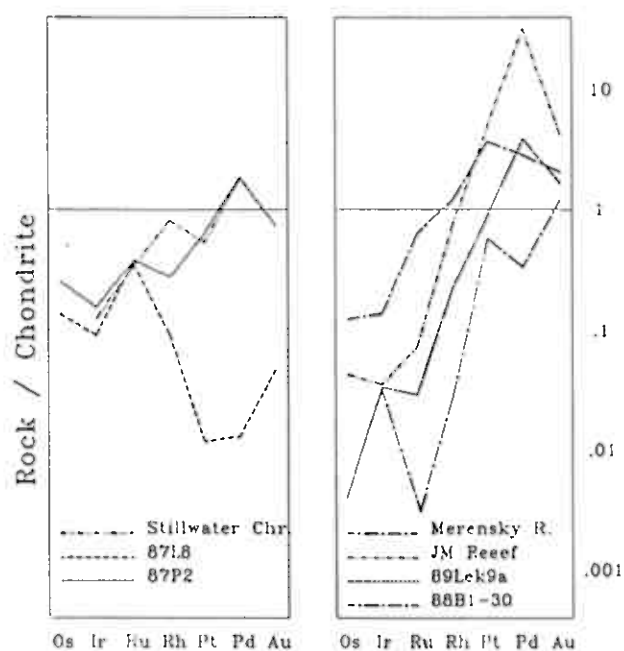
FIG. 20. Comparison of the PGE-patterns of the stratabound chromitites with chromitite from the Stillwater Complex (a), and of the PPGE-enriched horizons
