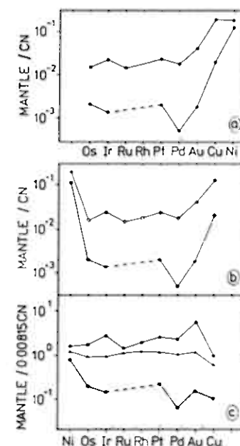
Fig. 1. (a) Conventional chondrite normalized metal patterns showing the range of rocks representing mantle (sources for mantle indicated in Appendix). Note that from Au to Ni the pattern is not flat. (b) Metal pattern of mantle fragments with Ni to the left of Os and Cu to the right of Au; chondrite normalized. Note the peaks at Ni and Cu which reflect the fact that there is 10–20 times more Ni and Cu chondrite normalized in the mantle than there are noble metals. If metal diagrams from ultramafic and mafic rocks are chondrite normalized they too will have peaks at Ni and Cu because they are mantle derived. (c) Revised metal pattern for the range of rocks representing mantle normalized to 2000 ppm for Ni 28 ppm for Cu and 0.008 15 \times chondrites for the noble metals. Note that the metal patterns are now flat (triangles indicate the average value from the data base).
