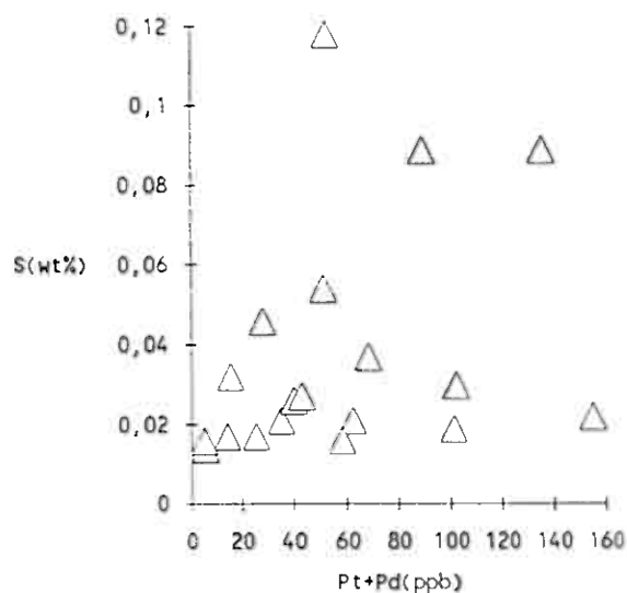
FIG. 17. Variation between S and Pt + Pd in core 88B4 taken across R6 between profile A and B.
