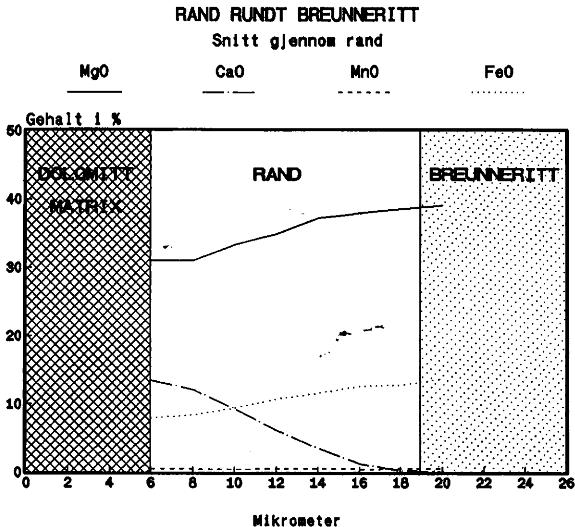
Figur 10. Scanning over rand rundt breunneritt.
