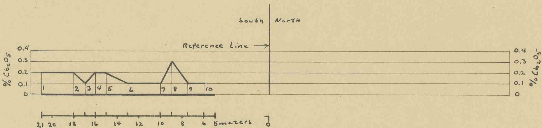
Trench 3 Assays 1-10
