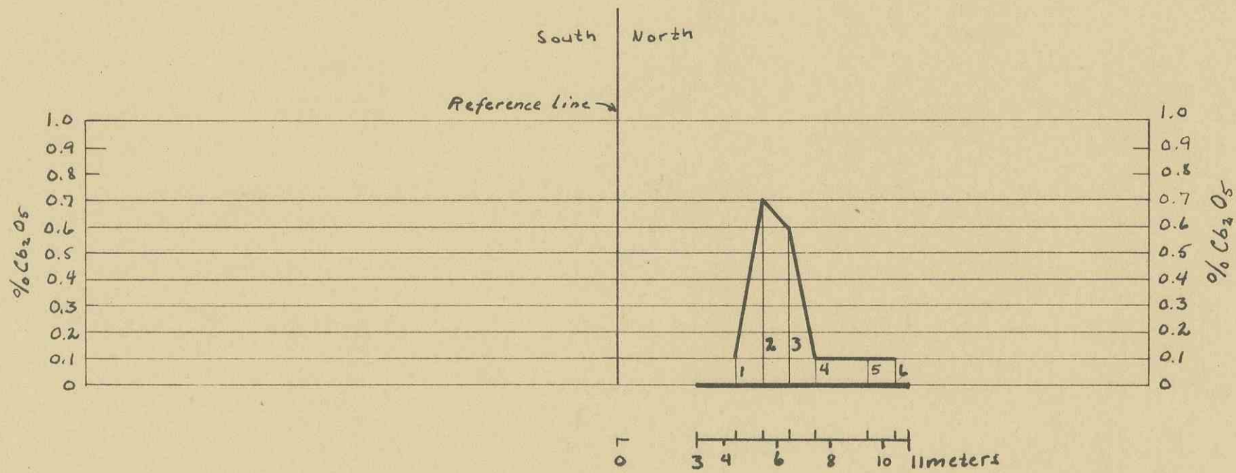
Trench 1 Assays 1-6
