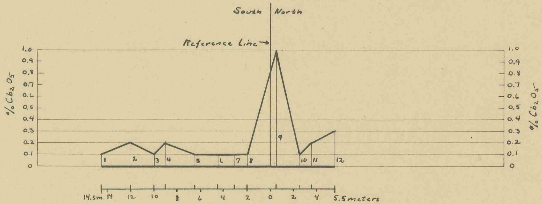
Trench 2 Assays 1-12
