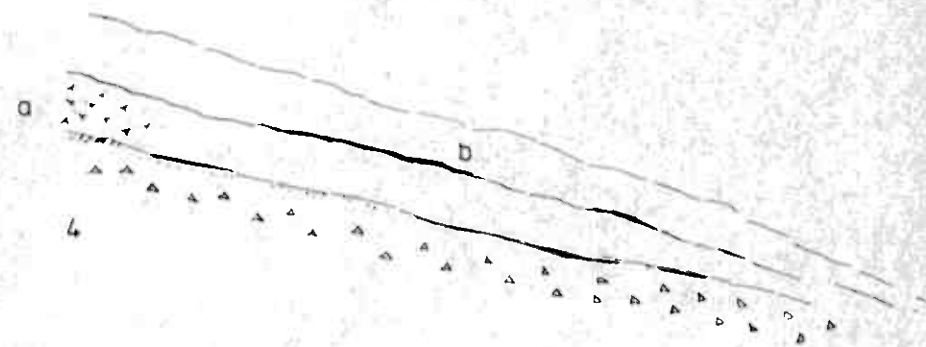
Possible origins of cherts occurring within homogeneous pillow flows as cusps (a) or horizons (b)
