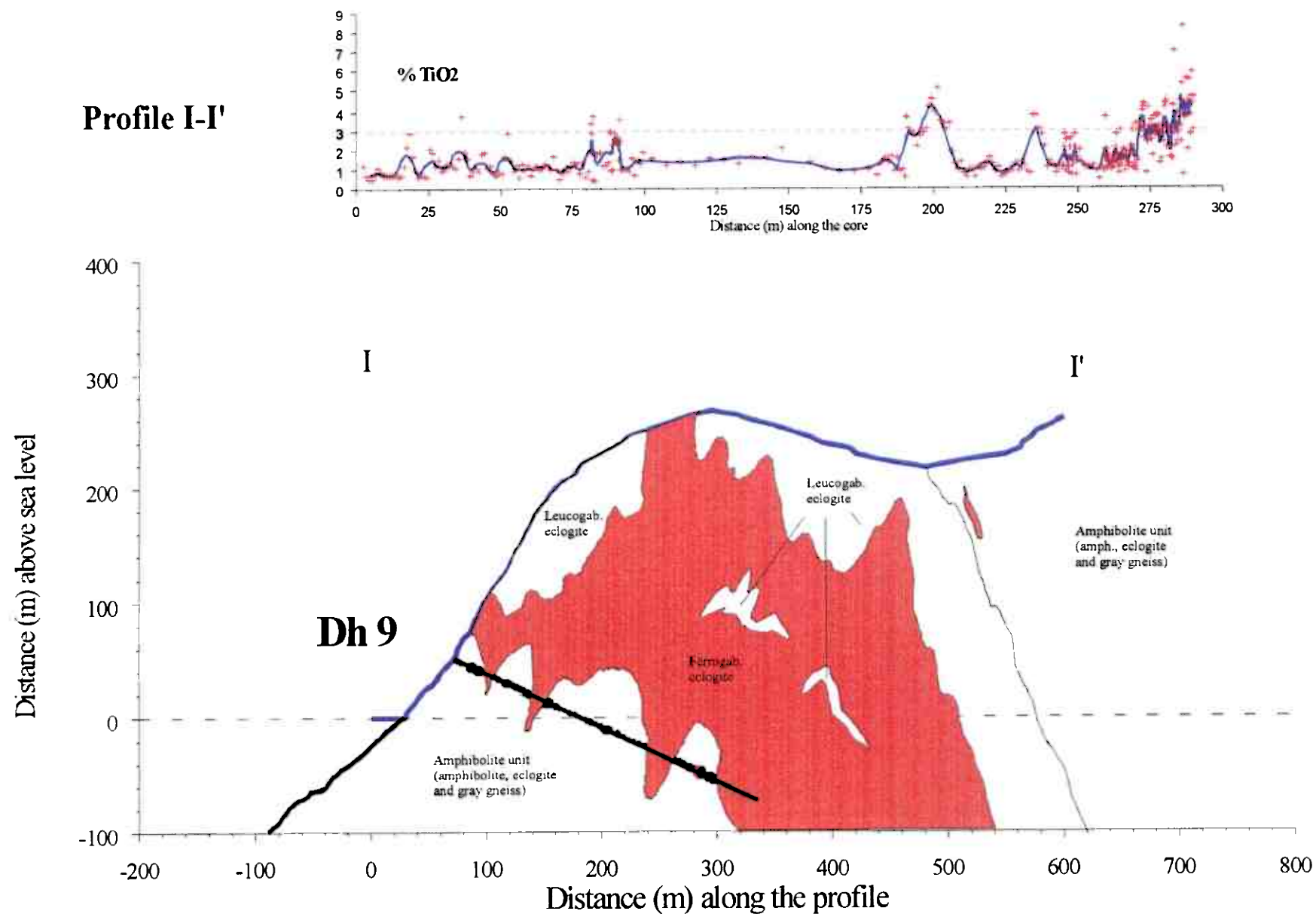
Fig. 10: Geologic profile showing the major geologic relations, the position of Dh9 in the profile and the \text{TiO}_2 -distribution along the bore-hole. The indicated geologic relations at depth are speculative.
