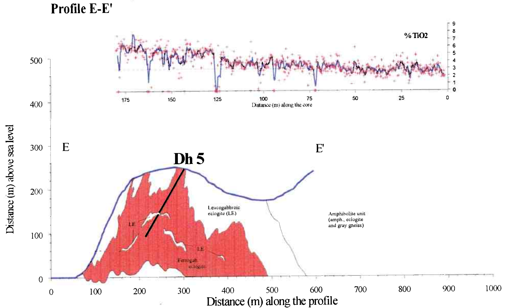
Fig. 6: Geologic profile showing the major geologic relations, the position of Dh5 in the profile and the \text{TiO}_2 -distribution along the bore-hole. The indicated geologic relations at depth are speculative.
