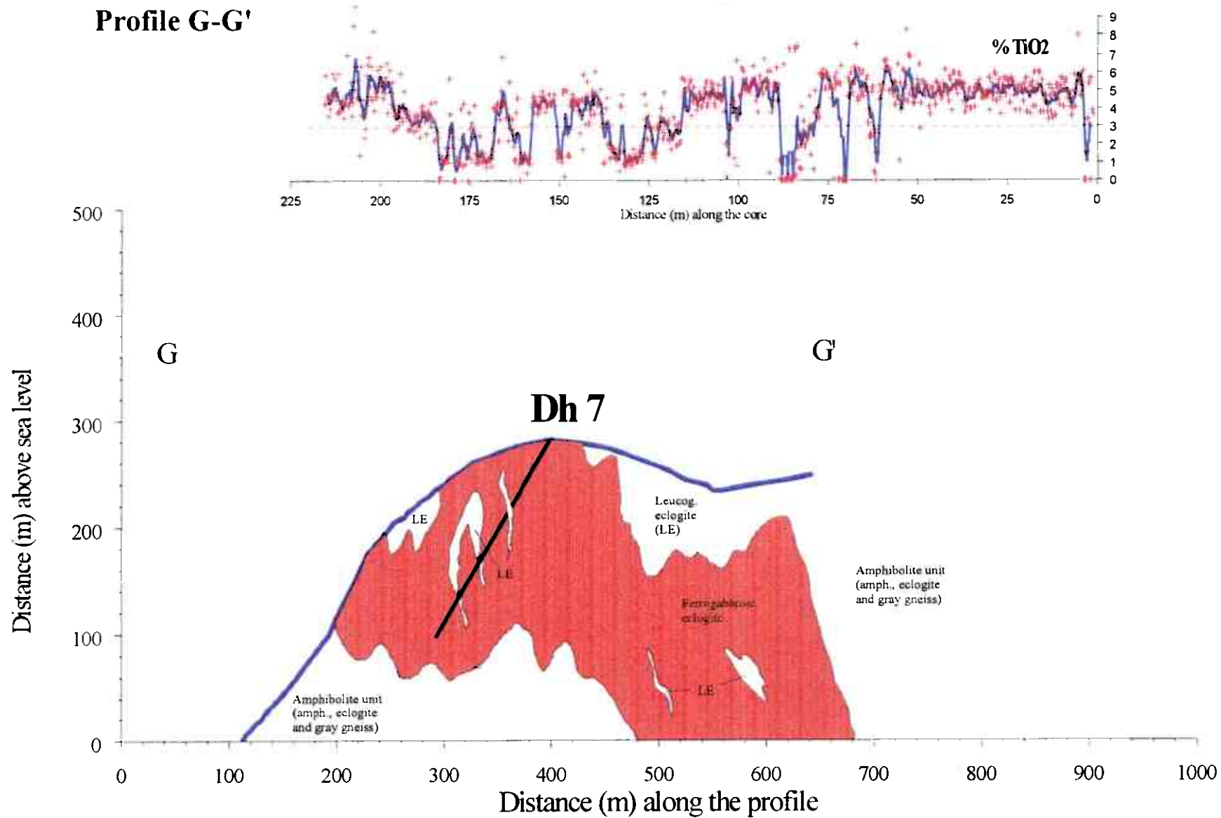
Fig. 8: Geologic profile showing the major geologic relations, the position of Dh7 in the profile and the \text{TiO}_2 -distribution along the bore-hole. The indicated geologic relations at depth are speculative.
