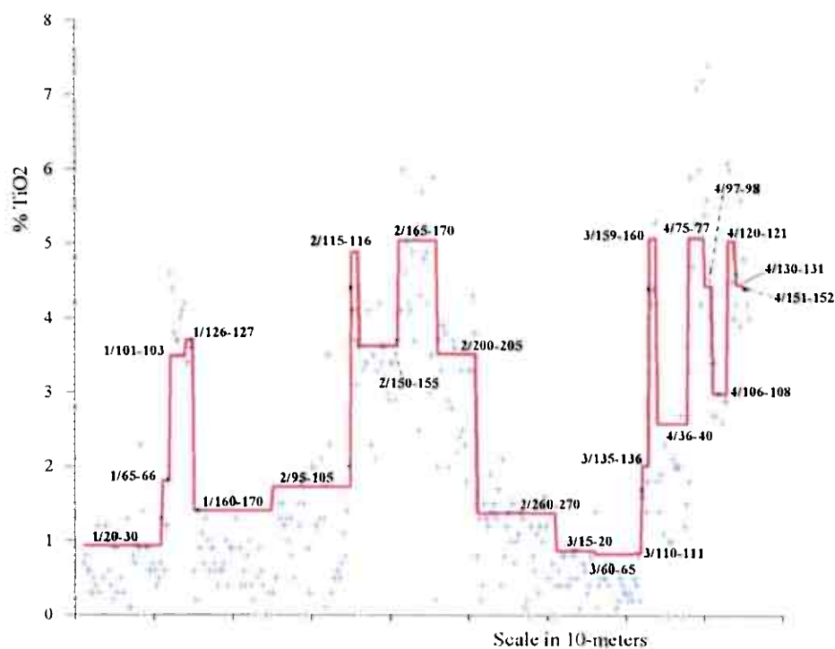
Fig. 21: Comparison of X-Met analyses of cores from Engbøfjellet (crosses) and XRF laboratory analyses (solid line) of the respective core sections.
