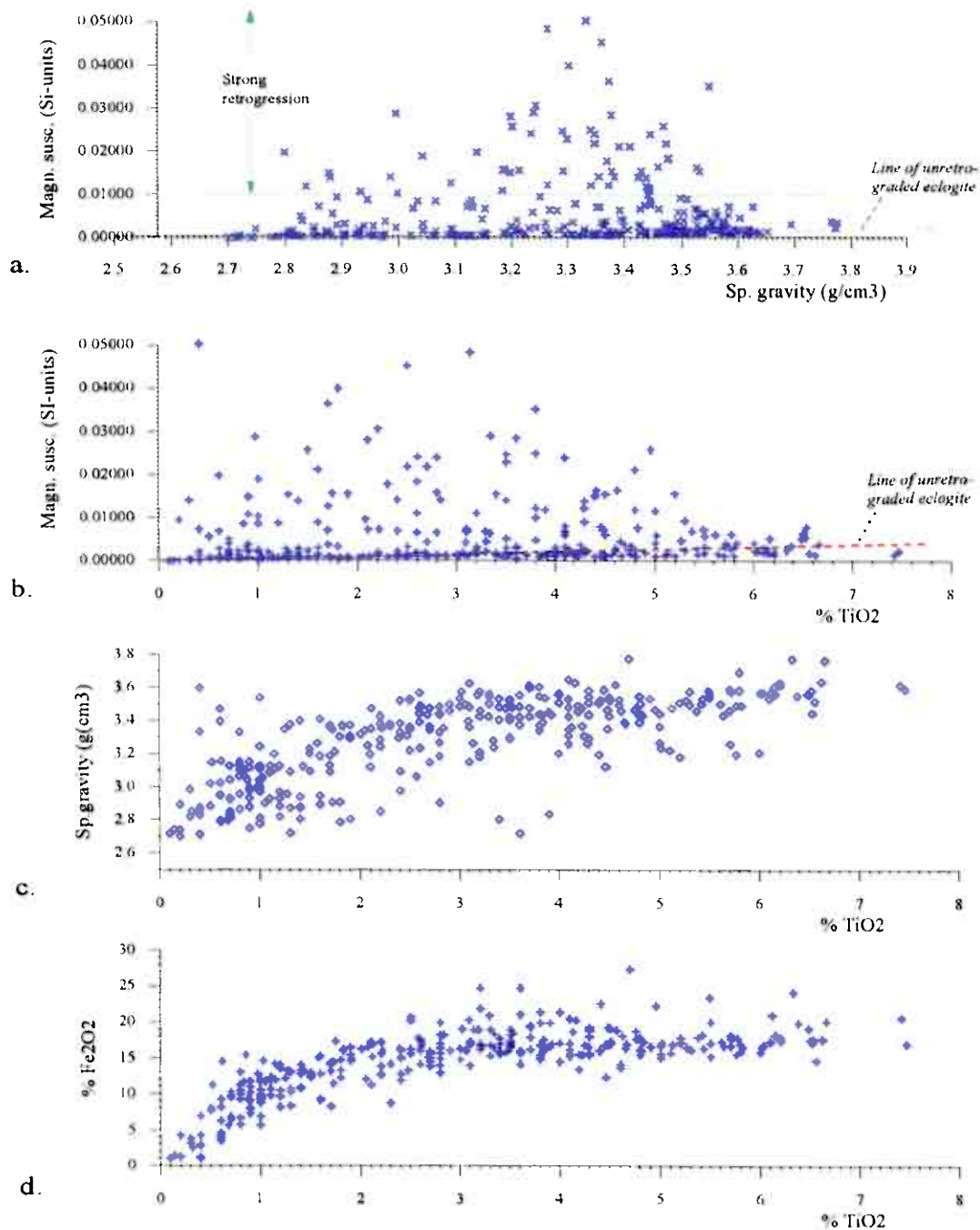
Fig. 24: Scattergram plots: (a) specific gravity vs. magnetic susceptibility, (b) % TiO 2 vs. magnetic susceptibility, (c) % TiO 2 vs. specific gravity, and (d) % TiO 2 vs. % Fe 2 O 3 . The high-magnetic character of some high density eclogites (<3 g/cm 3 ) is caused by secondary magnetite along retrogressive cracks in the eclogite; thus altogether, a relatively minor portion of these samples retrograded.
