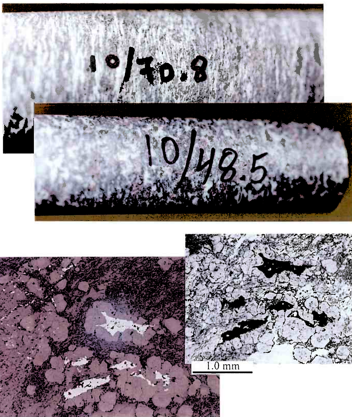
Fig. 16: Photographs of core and thin-section of leucogabbroic eclogite. Upper photo: representative, slightly sheared leucogabbroic eclogite from Dh10 at 70.8 m. Upper central photo: Massive leucogabbroic eclogite with preserved gabbroic texture from Dh10 at 48.5 m. Photo at lower right: microphotograph (thin section 10/46.9; reflected light) of rutile (black) in leucogabbroic eclogite. Garnet corona (around rutile) and fine-grained areas of clinozoisite + phengite + quartz + amphibole + omphacite after magmatic plagioclase are typical of partly recrystallized gabbroic textures. Photograph at lower left: same rutile grains (light gray; reflected light) as in the previous photo. The light gray patches in the left part of the photo are fine-grained rutile. Rutile in leucogabbroic eclogite normally occurs as fairly large grains or aggregates of grains and as scattered (dusty) grains as shown on this photograph. In retrograded leucogabbroic eclogites the fine-grained oxide dust is usually magnetite.
