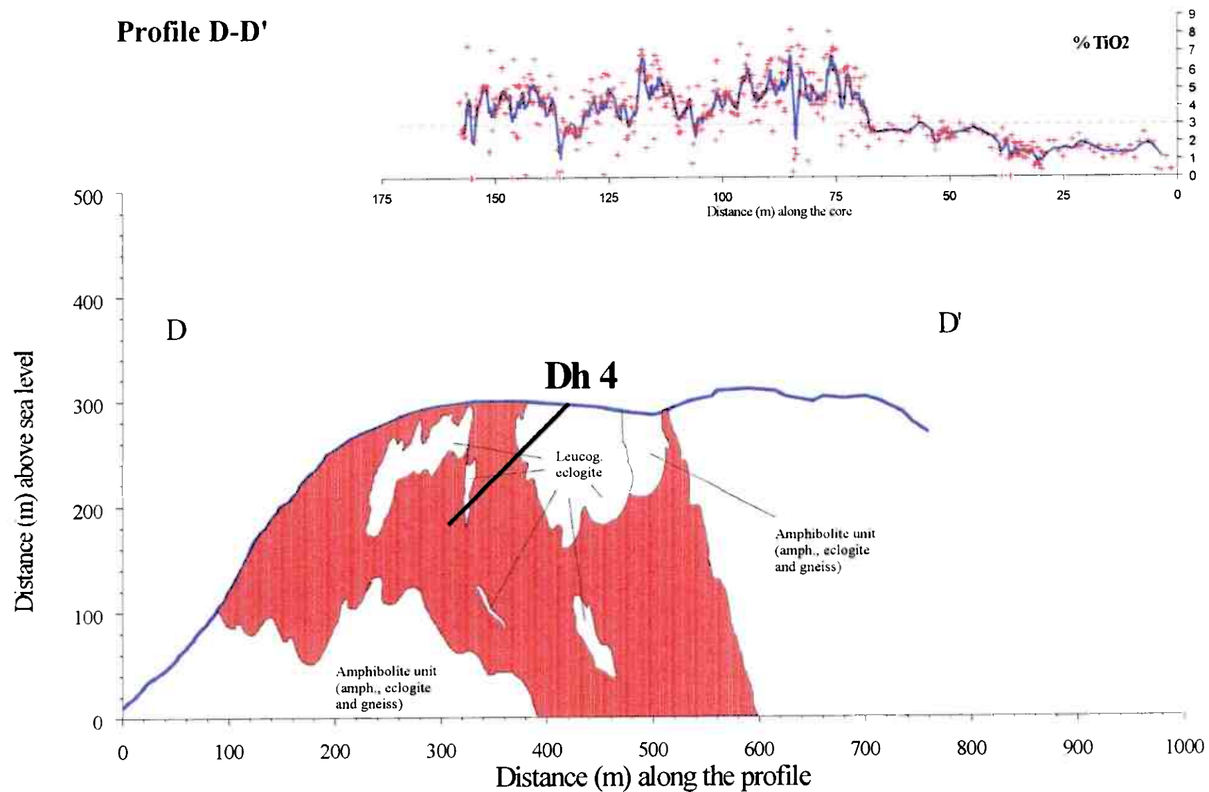
Fig. 5: Geologic profile showing the major geologic relations, the position of Dh4 in the profile and the \text{TiO}_2 -distribution along the bore-hole. The indicated geologic relations at depth are speculative.
