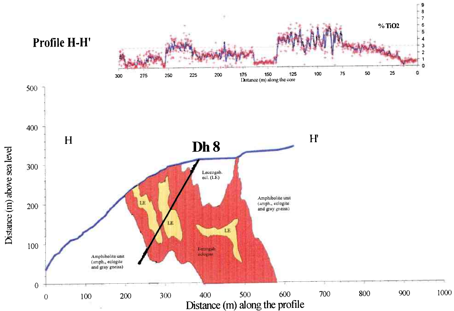
Fig. 9: Geologic profile showing the major geologic relations, the position of Dh8 in the profile and the \text{TiO}_2 -distribution along the bore-hole. The indicated geologic relations at depth are speculative.
