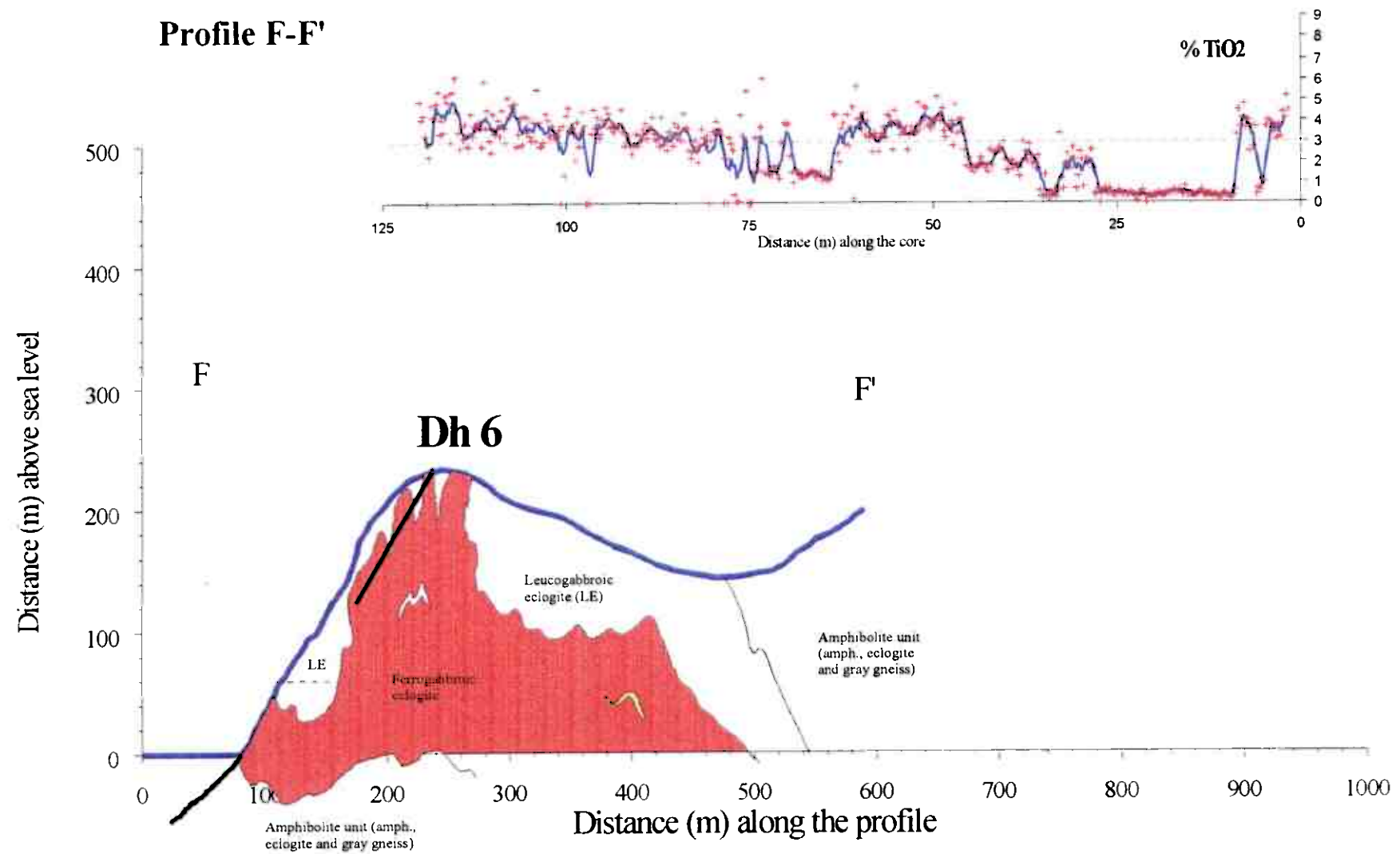
Fig. 7: Geologic profile showing the major geologic relations, the position of Dh6 in the profile and the \text{TiO}_2 -distribution along the bore-hole. The indicated geologic relations at depth are speculative.
