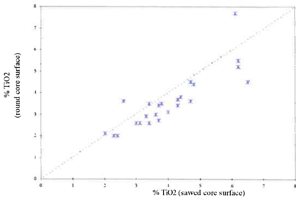
Fig. 22: TiO 2 -analyses on cut (sawed) core surface vs. round core surface by NGU's X-Met. Each plotted value is an average of 3 individual analyses (15 sec. counting time). See Appendix 3 for further analytical details.
