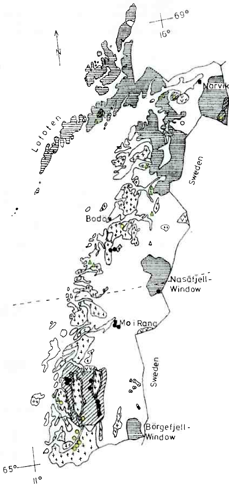
Regional Geology Map of Nordland
