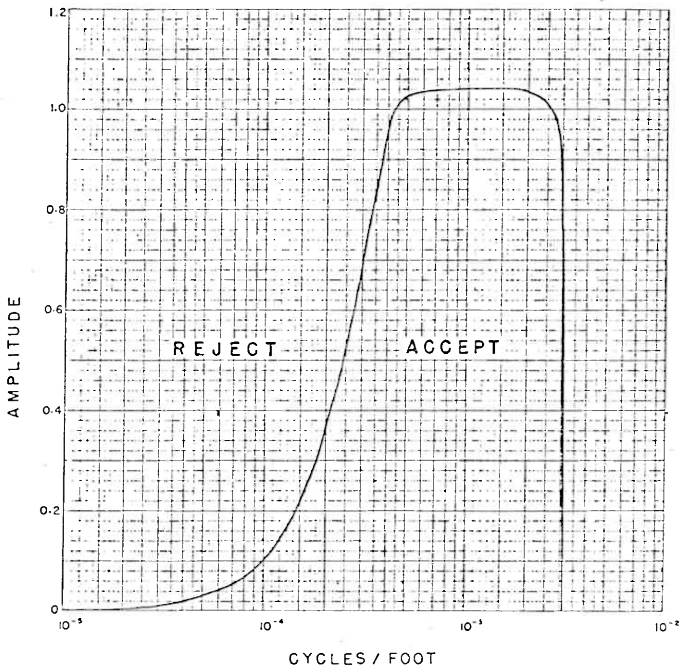
Figure 3 Frequency response of VLF-EM operator
